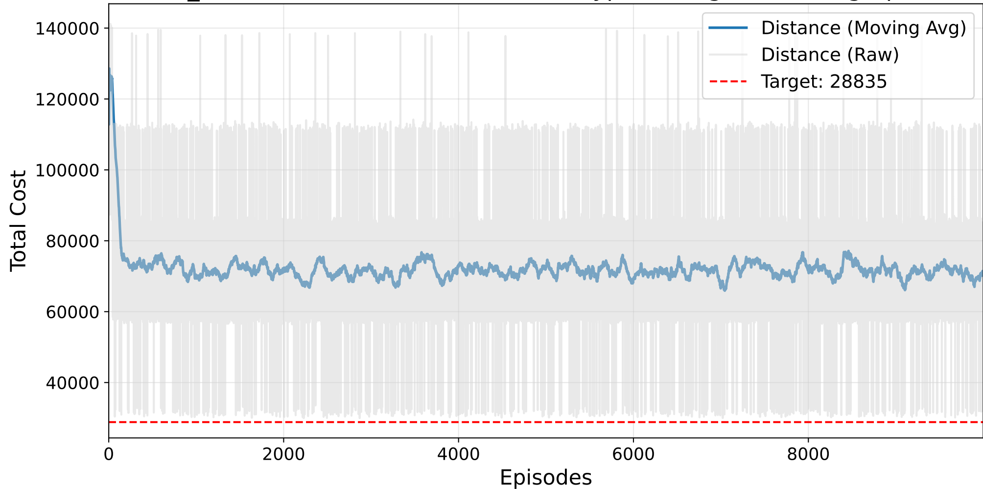
Final NO_BAYESIAN Masked AutoRL-SOP (HyperTuningSK) Training - p43.3.sop
